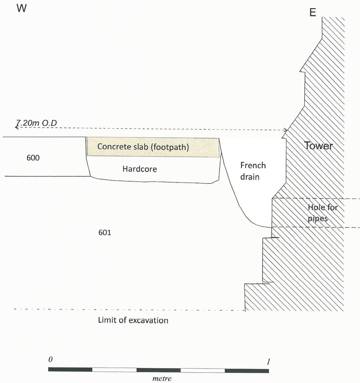
Fig. 14 Profile of tower west wall showing position of hole drilled for service pipe. Scale 1:10
